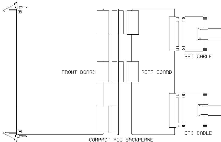
Figure 4: Installing Cables on J1 and J2
